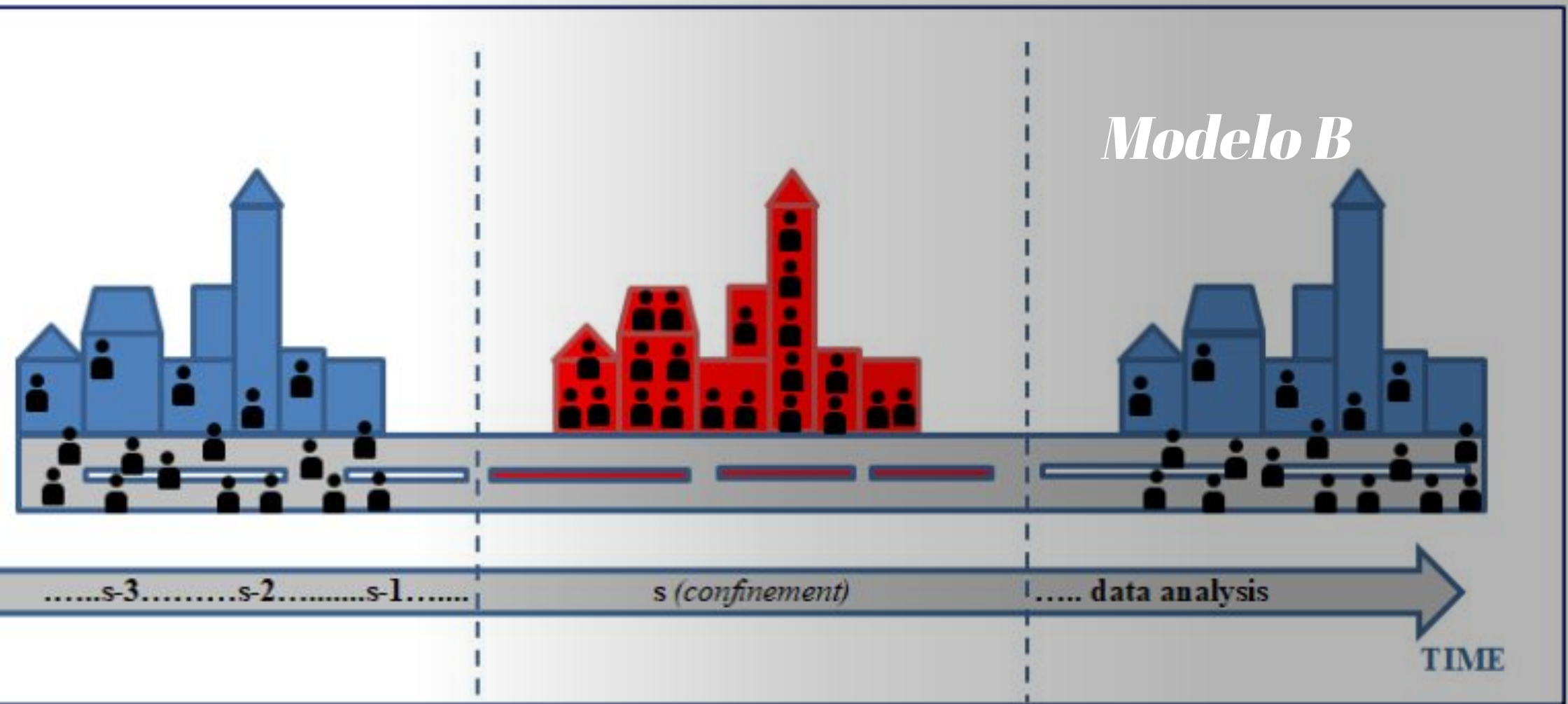
Figure 2 : The second way to study the effectiveness or not of the confinement (one city). s-3 : season of the flu 3 years before the confinement. s-2 : season of the flu 2 years before the confinement. s-1 : season of the flu 1 year before the confinement.
